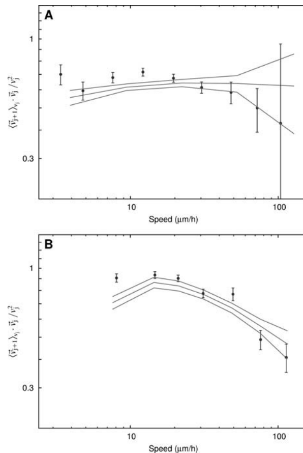
FIGURE 12 Expectation value of \vec{v}_{j+1} for given \vec{v}_j , projected onto the latter, and measured in units of the latter's length, i.e., \langle \vec{v}_{j+1} | \vec{v}_j \rangle \cdot \vec{v}_j / v_j^2 as function of |\vec{v}_j| . Here \vec{v}_j and \vec{v}_{j+1} are consecutive velocities computed from positions measured with 15-min time lapses; see Appendix A. In the OU model, the quantity plotted here is constant, independent of speed. (A) Data points are experimental values from HaCaT cell trajectories. Their consistency with a constant value suggests a linear velocity dependence of the noise-averaged acceleration in a HaCaT model. Thick curve surrounded by two thin curves is the theoretical result for same quantity, \pm 1 SD, computed from HaCaT model in Eq. 6 fitted to data shown in Fig. 4, B, E, and F, and here. It's small, but nonvanishing dependence on speed, is due to a combination of time-lapse sampling and speed dependence of the model's noise term. (B) Data points are experimental values from NHDF cell trajectories. Their distinct speed dependence suggests a nonlinear velocity dependence of the acceleration in an NHDF model. Thick curve surrounded by two thin curves is the theoretical result for same quantity, \pm 1 SD, computed from the NHDF model fitted to data shown in Fig. 5, B, E, and F, and here.
